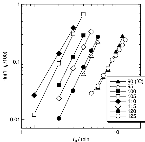
Fig. 7. Avrami plots of PLLA-0 film (process A).
